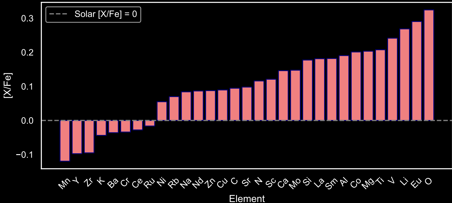
Abundance Pattern for GALAH Red Giants: Star Field [67] (N=82)
