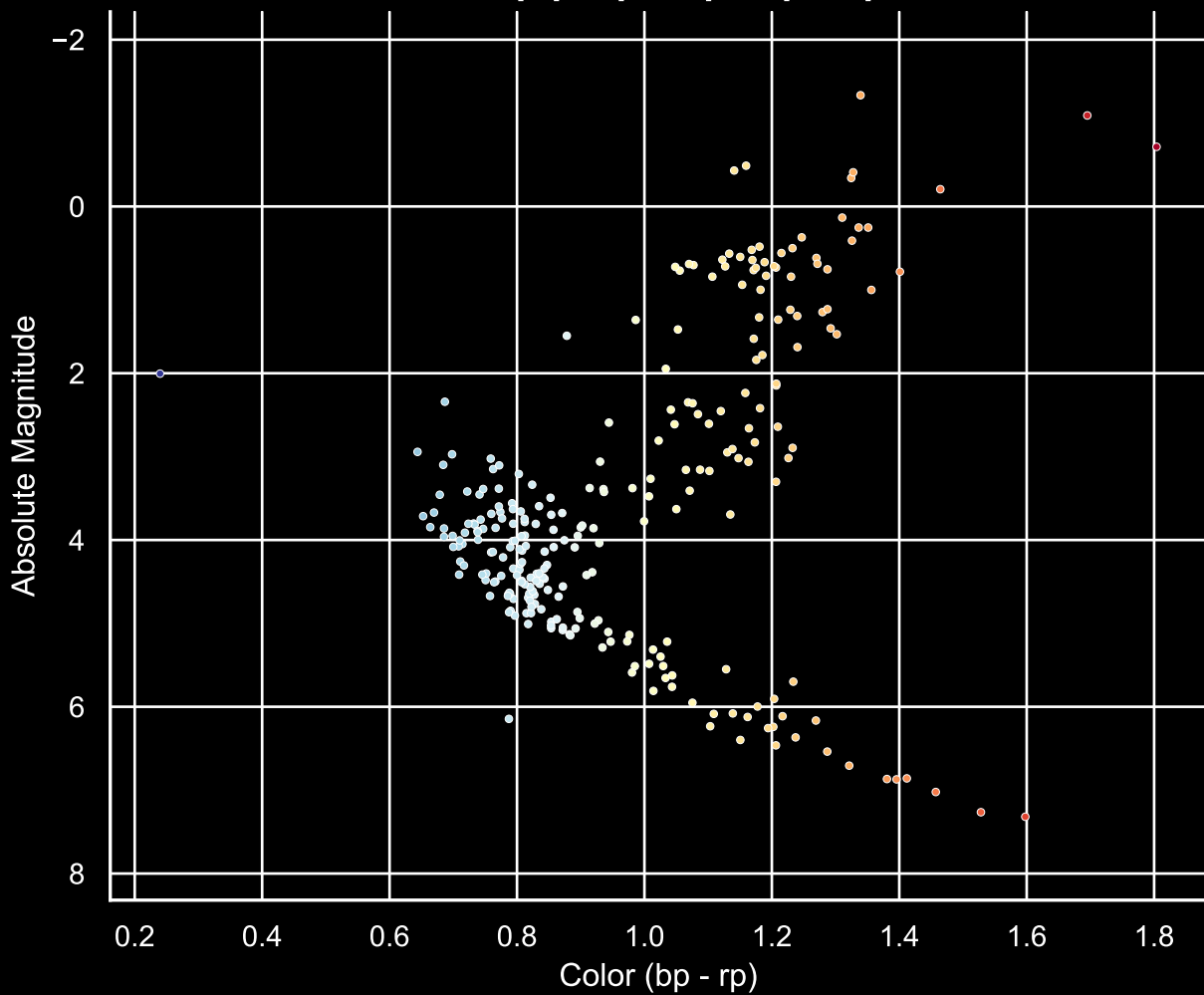
GALAH Hertzprung-Russel Diagram Field [67] Ra [325.23] Dec [-60.35]
