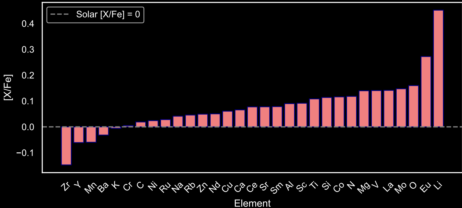
Abundance Pattern for GALAH Star Field [67] (N=272)
