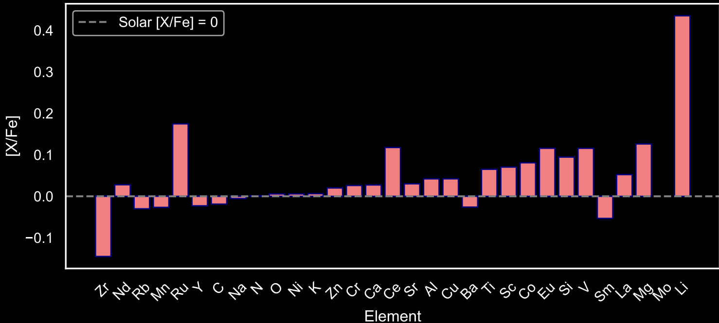
Abundance Pattern for GALAH Main Sequence Stars: Star Field [67] (N=123)
